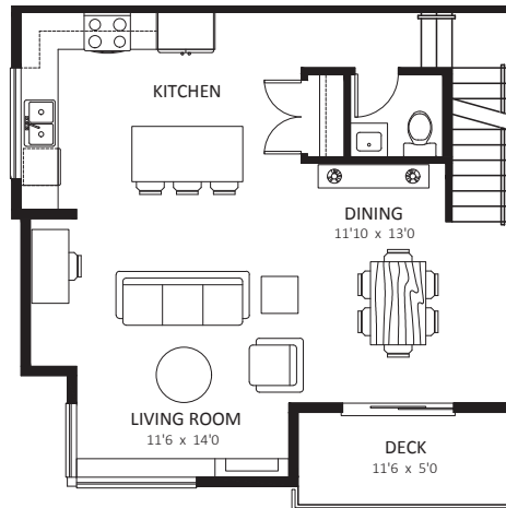
Main Level
