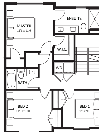
Upper Level
